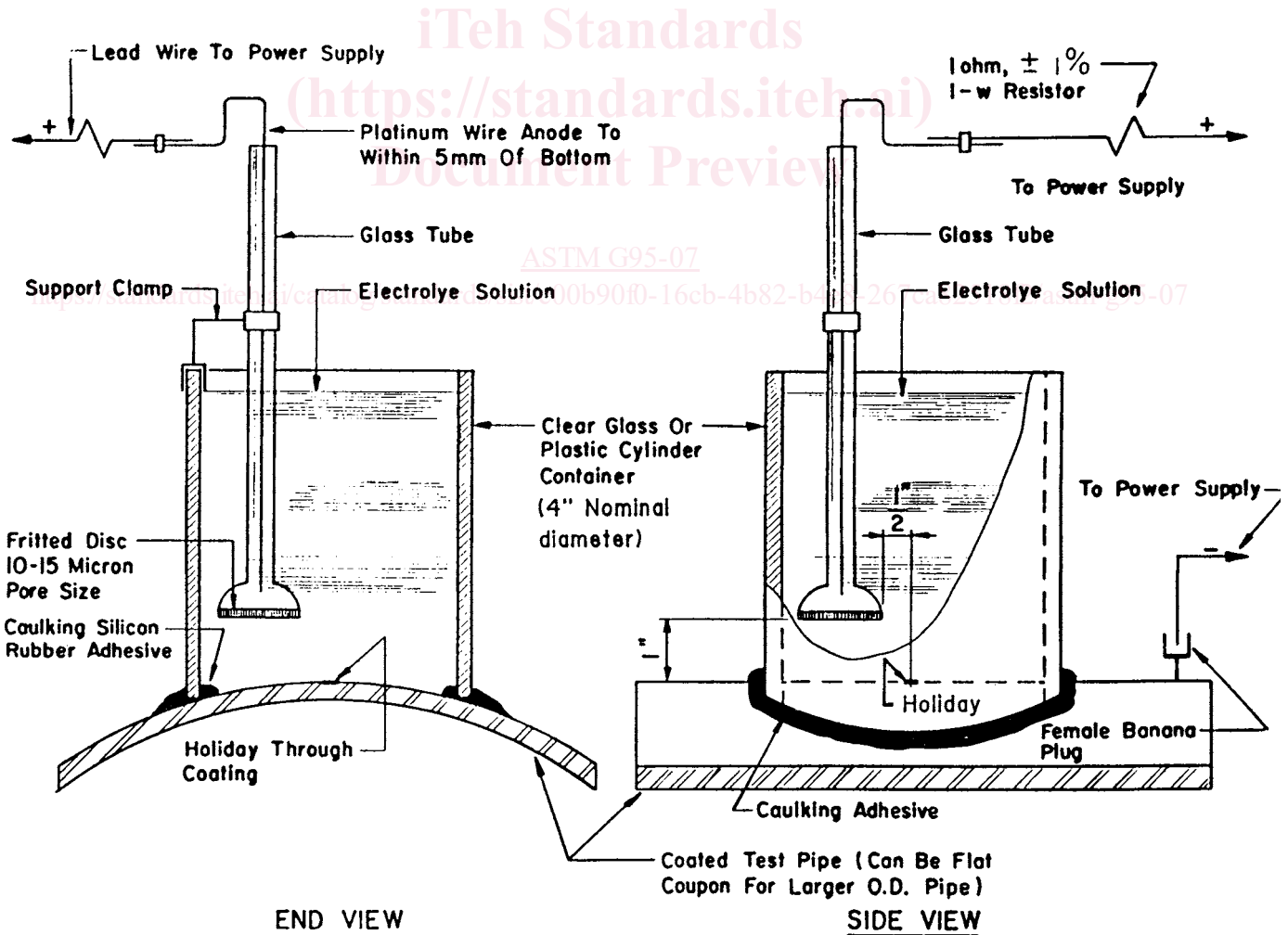
FIG. 1 Typical Test Set Up
