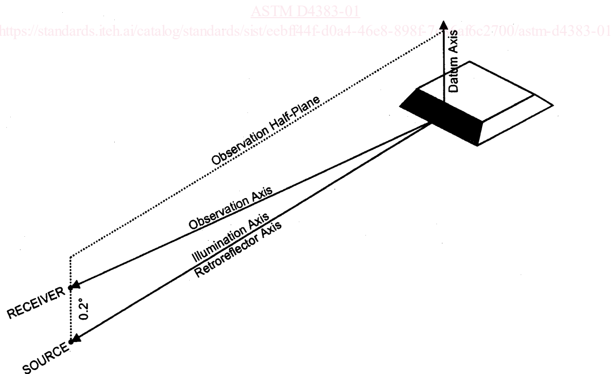
FIG. 2 Position of Marker for Photometry, 0° Entrance Angle
