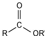
Figure A.2 — Liaison ester
