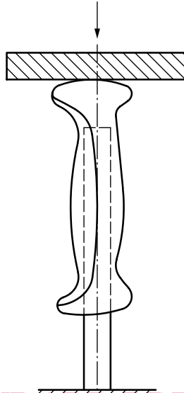
Figure 3 — Test arrangement for piercing resistance
