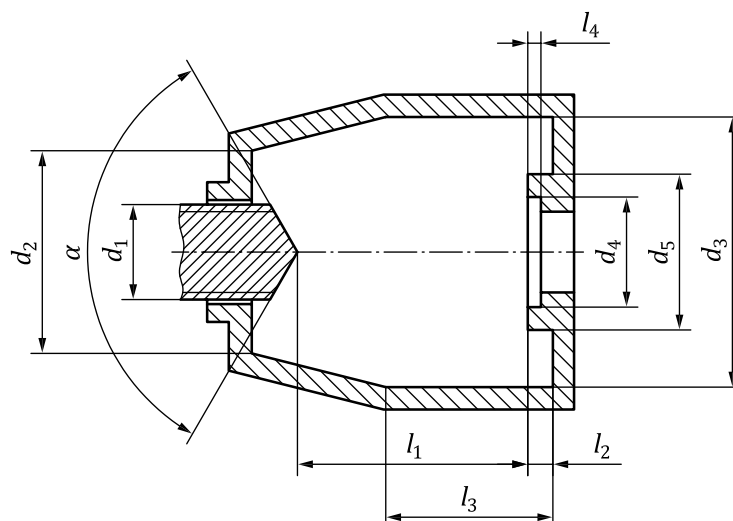
Figure 3 — Dimensions de l'étrier
