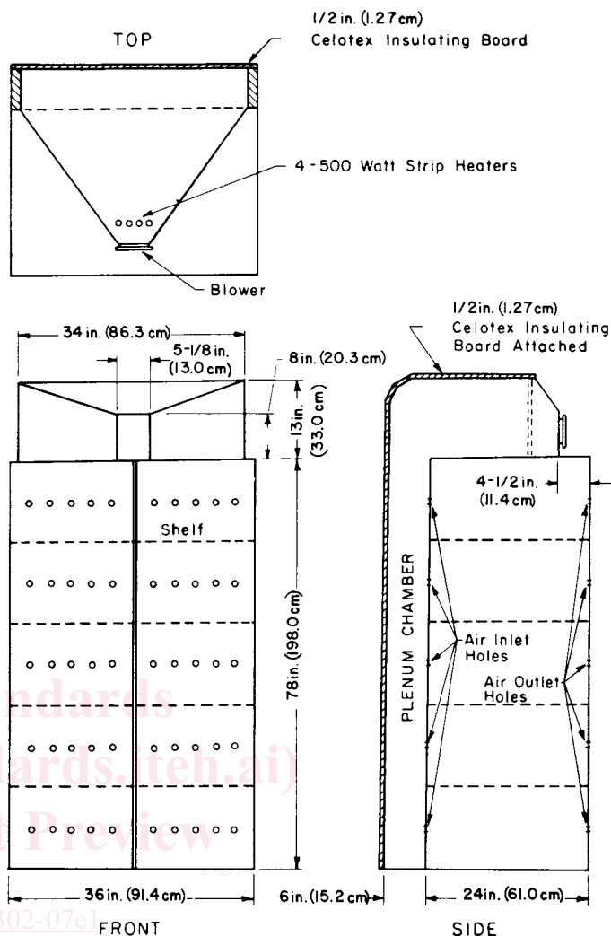
FIG. 2 Air-Drying Oven - d3302-07e1
