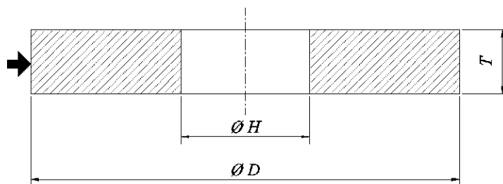
Figure 1 — Straight Wheel, Type 1
