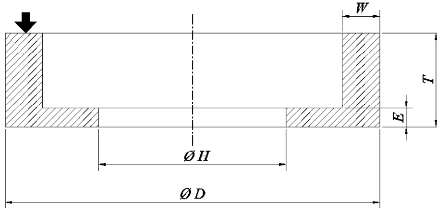
Figure 2 — Straight Cup Wheel, Type 6
