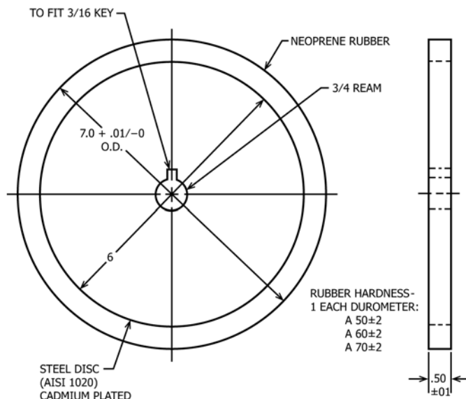
FIG. 2 Rubber Wheel
