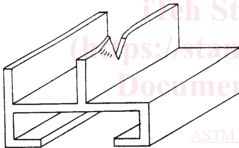
Tear - ductile - crack not sharp - tip of crack has greater than zero degree angle NON-FAILURE
