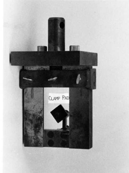
FIG. 2 Holding Block
