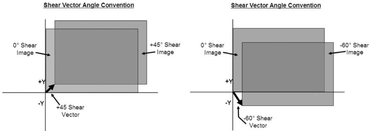
FIG. 1 Shear vector angle convention: Starting with the shear camera adjusted for a 0° shear condition, the sheared image is moved to the right (+X) or up/down, never adjusted in the direction of -X. For a +45° shear vector, the image is moved in the +X and +Y direction. For 60° shear vector, the image is adjusted in the +X and -Y directions. The convention allows determination of deformation direction from the unwrapped phase map.
