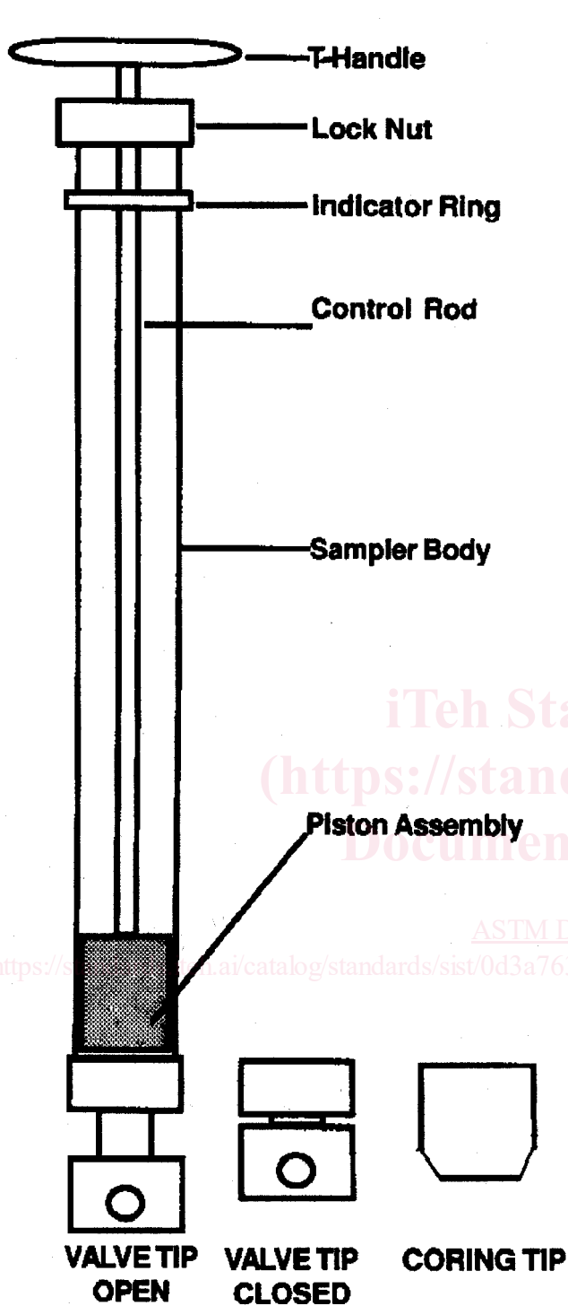
FIG. 5 Syringe Sampler
