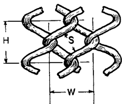
FIG. 1 Mesh Dimensions for 5/8-in., ½-in., and 3/8-in. Fabric
