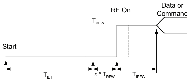
Figure 2 — RF detection and initial RF generation for PCD MODE and VCD MODE (standards.iteh.ai)
