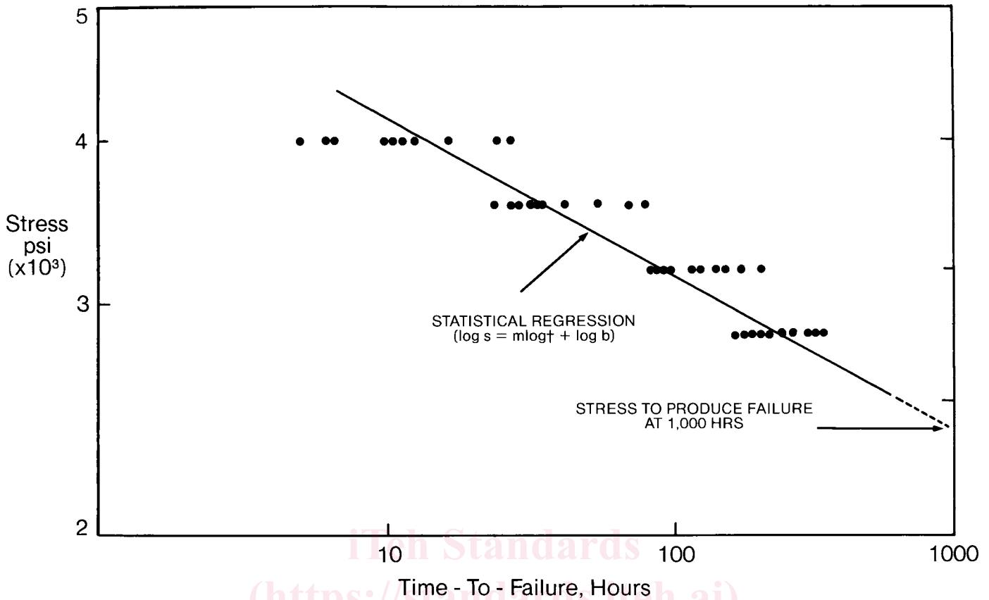
FIG. 4 Logarithmic Time-to-Failure (Stress Rupture) Curve
