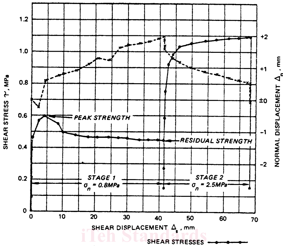
FIG. 1 Shear Stress - Displacement Graphs
