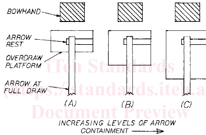
FIG. 2 Increasing Levels of Arrow Containment, Horizontal Plane
