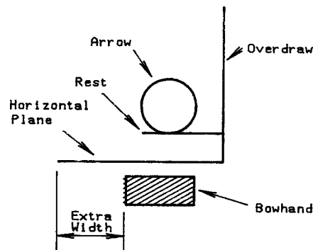
FIG. 3 Extended Width of the Horizontal Plate
