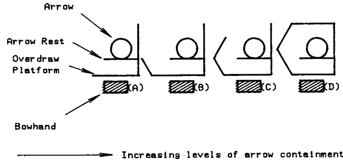
FIG. 1 Increasing Levels of Arrow Containment, Vertical Plane
