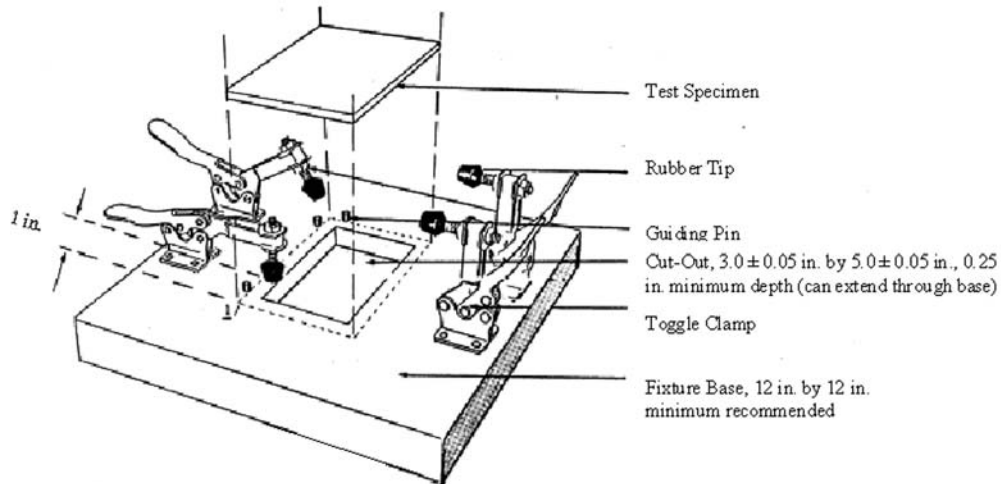
NOTE—Clamp tip centered 0.25 in. from edge of cut-out. FIG. 1 Impact Support Fixture (Inch-Pound Version)
