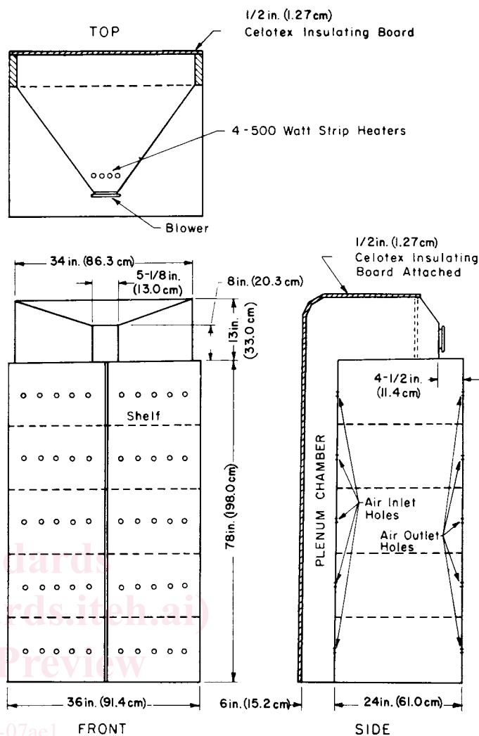
FIG. 2 Air-Drying Oven
