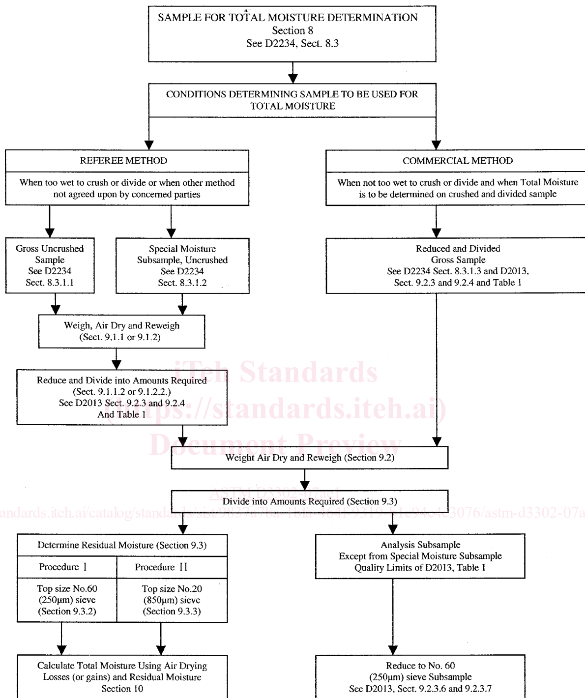
FIG. 1 Total Moisture Determination on Gross Sample, Special Moisture Subsample, or on Crushed and Divided Sample
