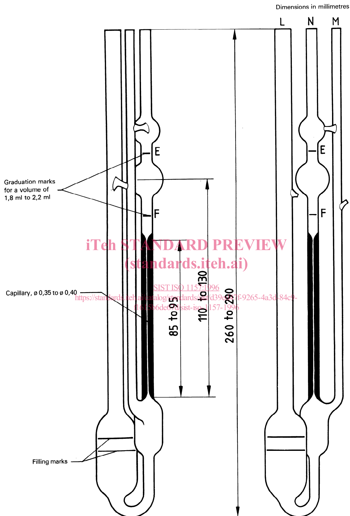
Figure 1 — Ubbelohde viscometer
