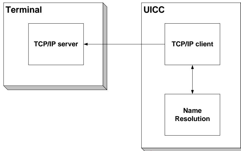
Figure 1: Local TCP/IP Client on UICC
