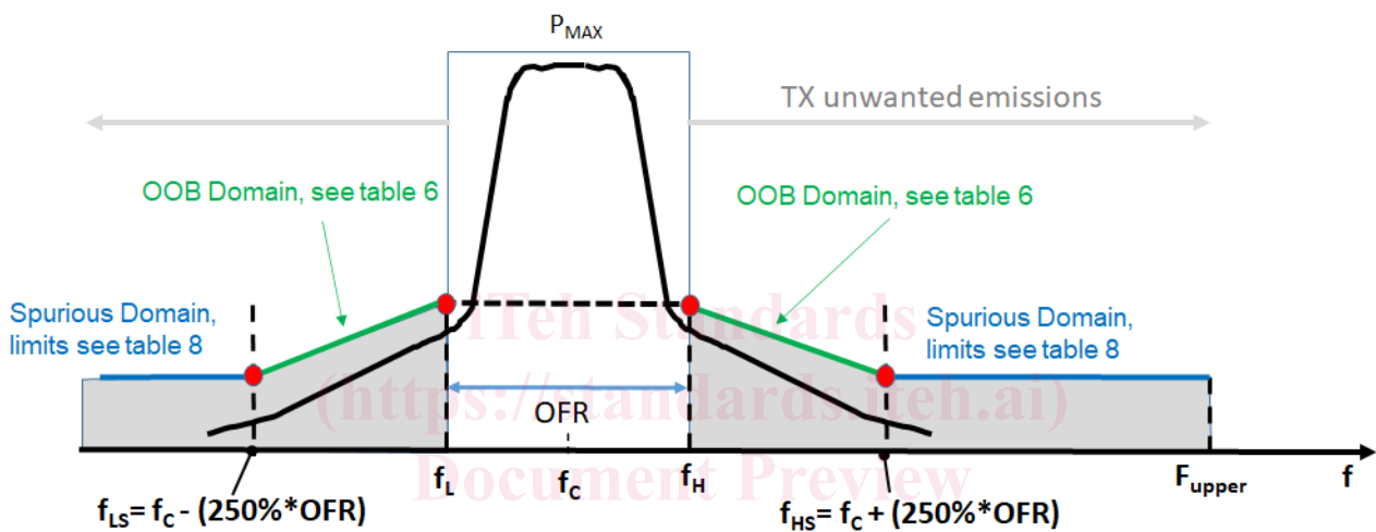
Figure 1: TX unwanted emissions within the OOB and Spurious Domain for GBSAR EUT
