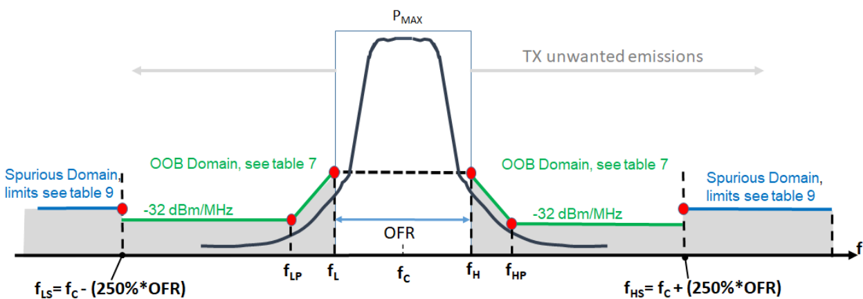
Figure 2: TX unwanted emissions within the OOB and Spurious Domain for HD-GBSAR EUT
