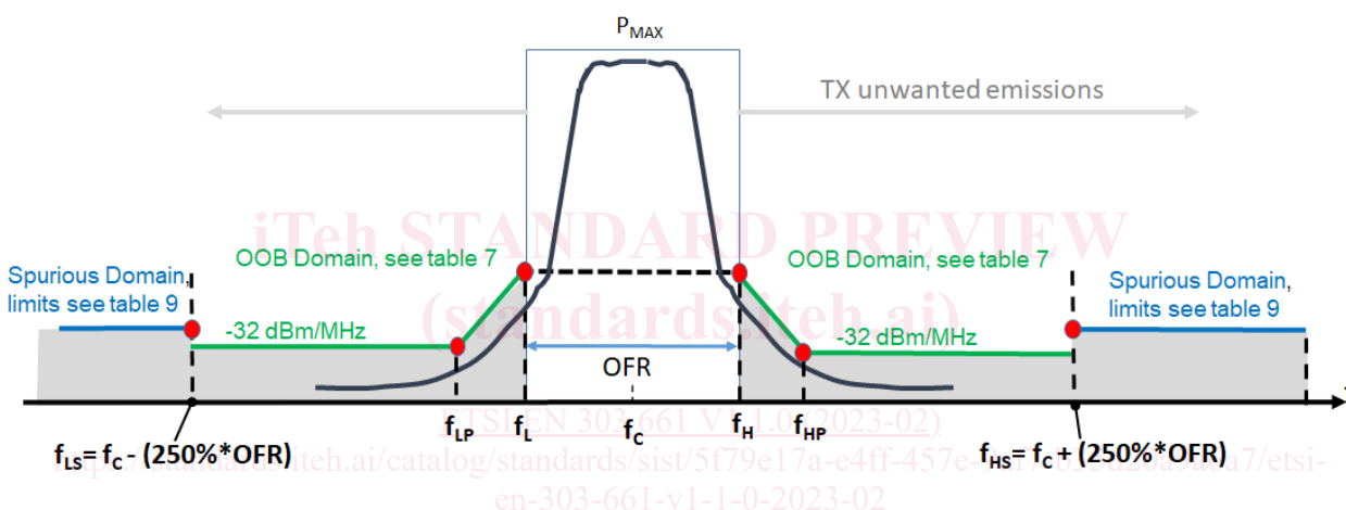
Figure 2: TX unwanted emissions within the OOB and Spurious Domain for HD-GBSAR EUT
