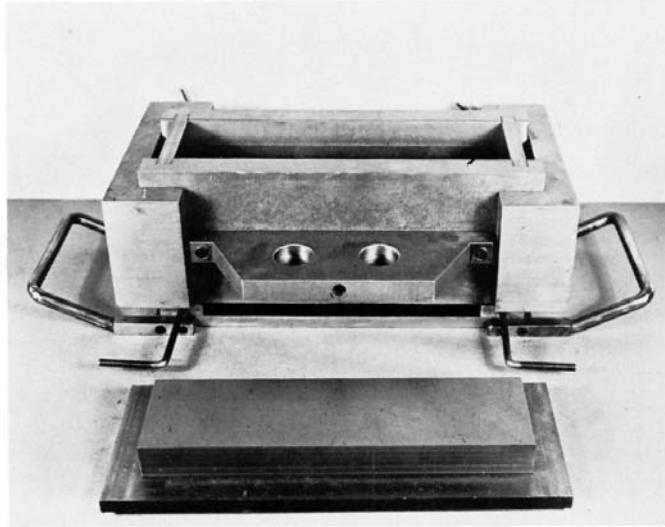
FIG. 3 Heavy Steel Mold and Top Plate for Making 3 by 3 by 11¼-in. (76.2 by 76.2 by 285.8-mm) Flexure Test Beam
