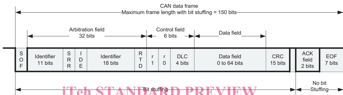
b) CAN extended frame format
