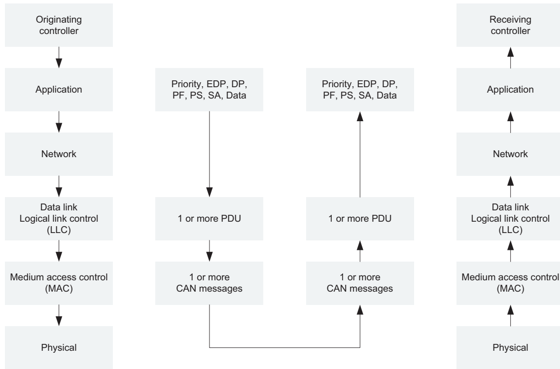
Figure 2 — Application of OSI model according to ISO 11783 (standards.iteh.ai)
