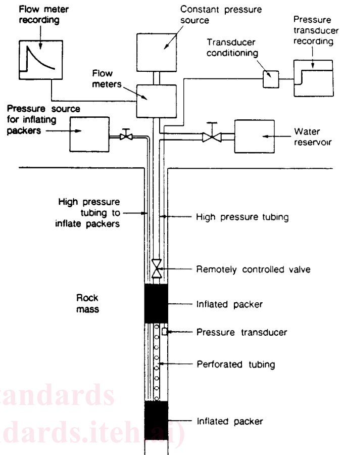
FIG. 1 Equipment Schematic
