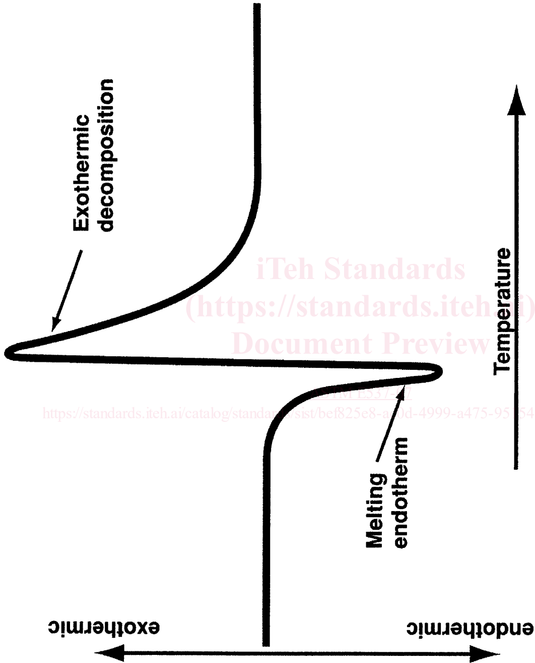
FIG. 2 DSC Curve Illustrating a Melting Process Immediately Followed by an Exothermic Decomposition
