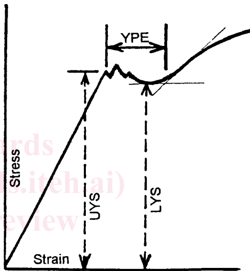
FIG. 2 Stress Strain Diagram Showing Yield Point Elongation and Upper and Lower Yield Strengths
