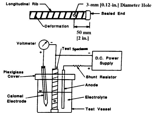
FIG. A1.1 Cathodic Disbondment Test Equipment Configuration
