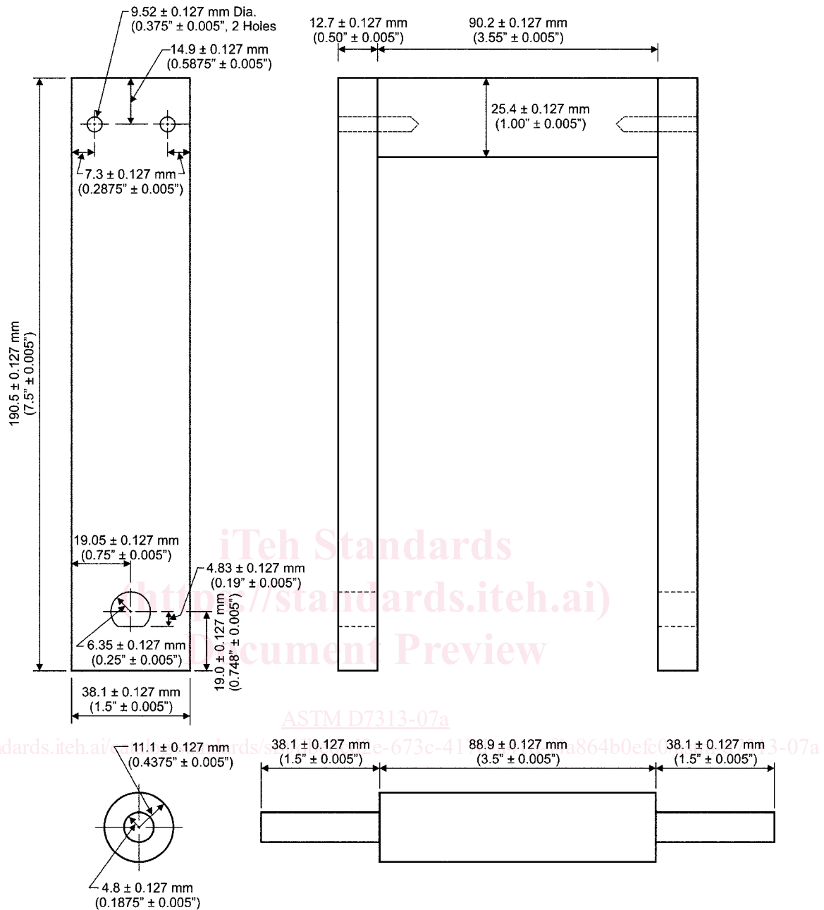
FIG. 1 Schematic of Loading Clevis
