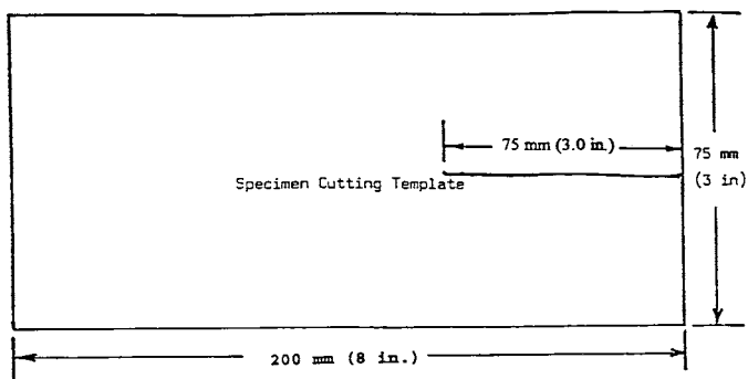
FIG. 1 Template for Marking and Cutting Tongue Tear Specimens, All Tolerances ±0.5 %
