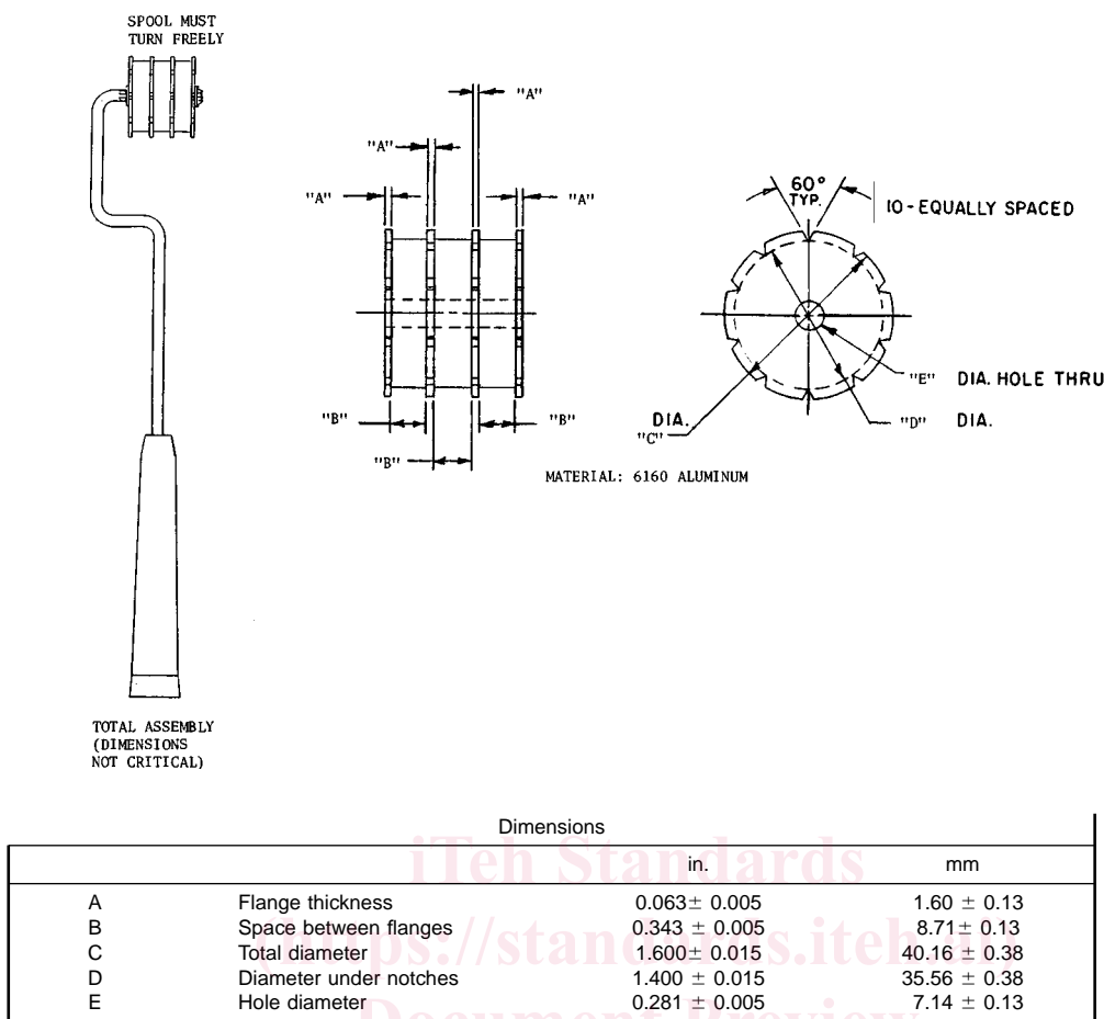
FIG. 1 Notched Spool Roller
