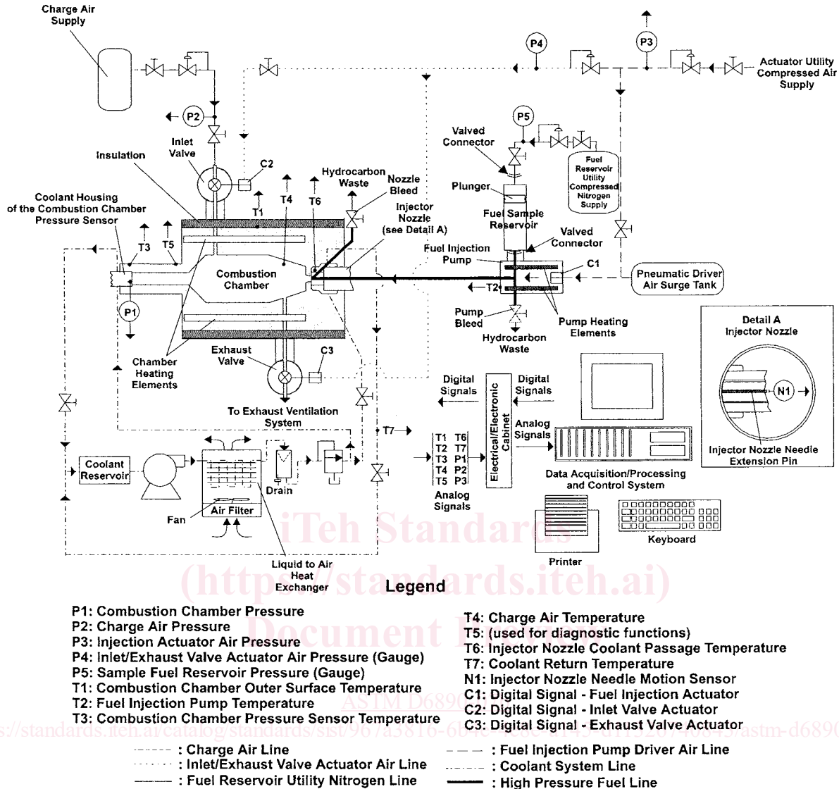
FIG. 1 Combustion Analyzer Schematic
