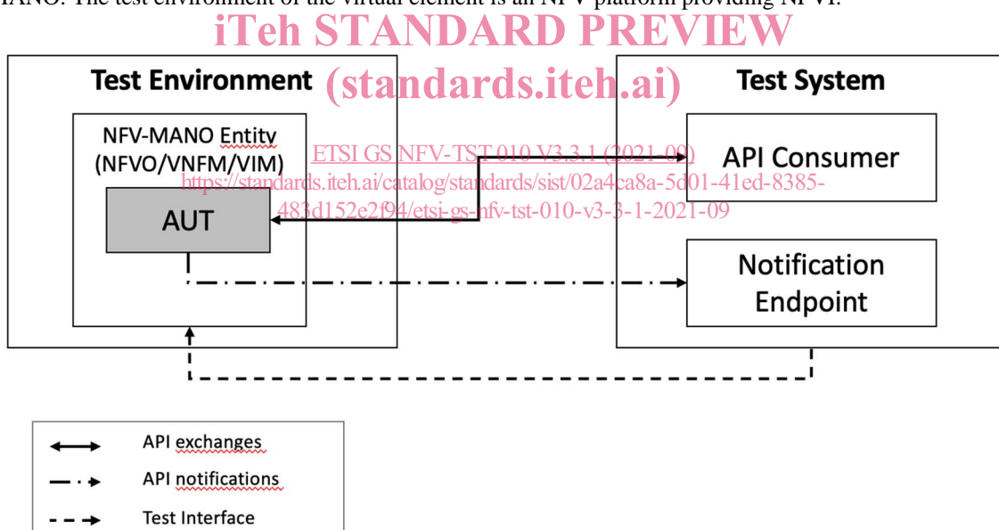
Figure 4.3.7-1: Configuration for tests of APIs with NFV-MANO as Producer
