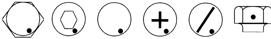
FIG. 1 Significant Surfaces on Externally Threaded Fasteners
