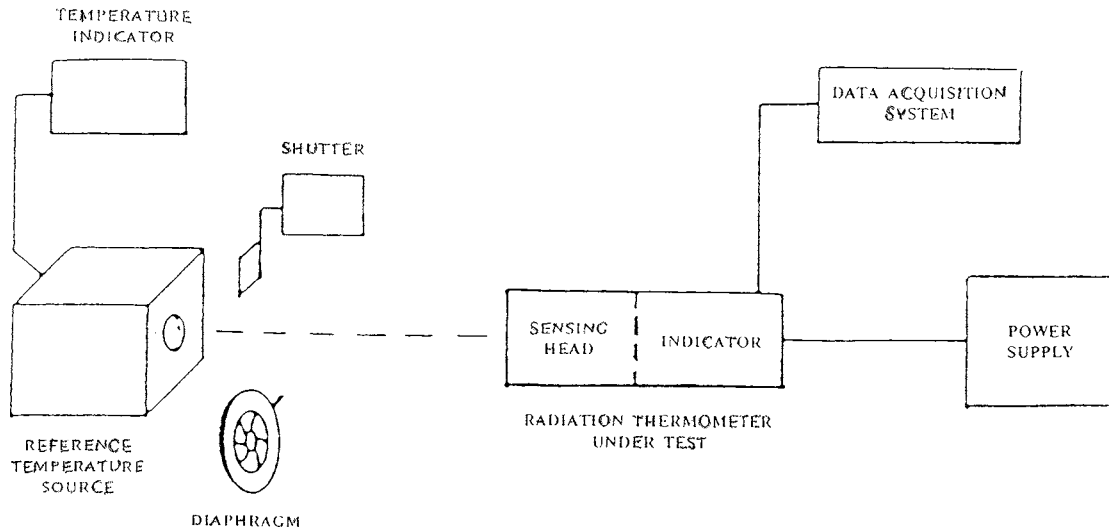
FIG. 2 Test Method Apparatus
