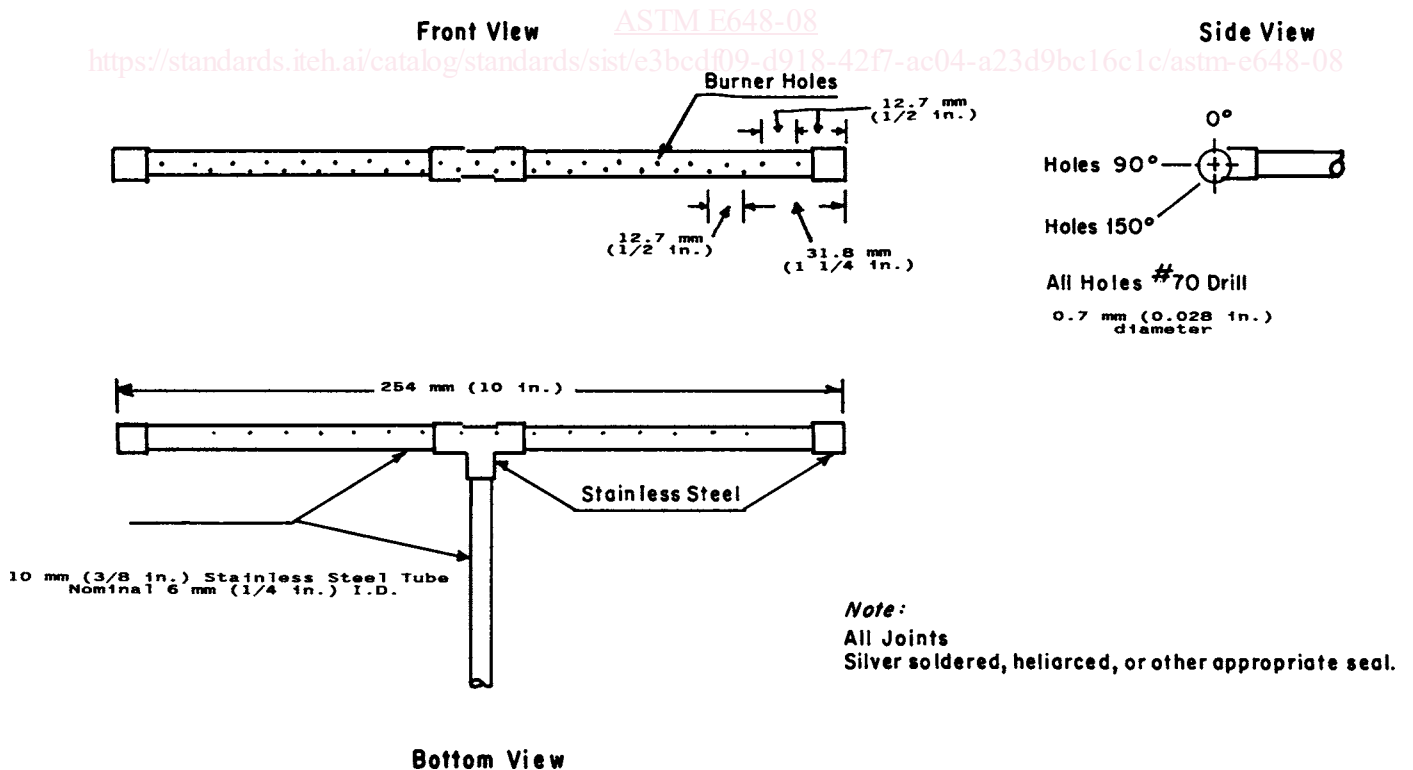
FIG. 6 5 Pilot Burner
