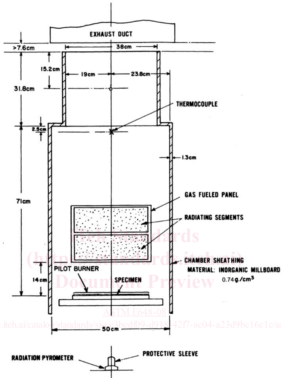
FIG. 5.4 Flooring Radiant Panel Tester Schematic Low Flux End, Elevation
