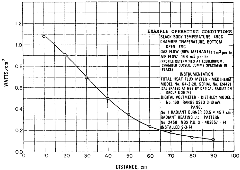
FIG. 3 2 Standard Radiant Heat Energy Flux Profile
