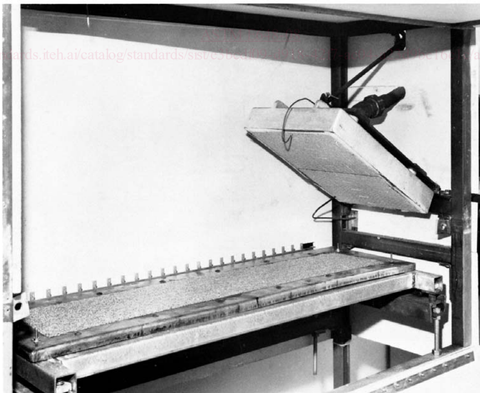
FIG.-2_1 Flooring Radiant Panel Test Showing Carpet Specimen and Gas Fueled Panel
