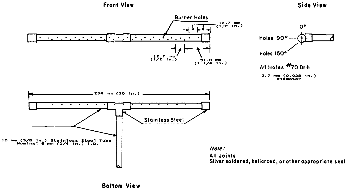
FIG. 5 Pilot Burner
