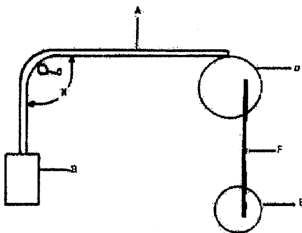
FIG. 1 Webbing Abrasion Tester
