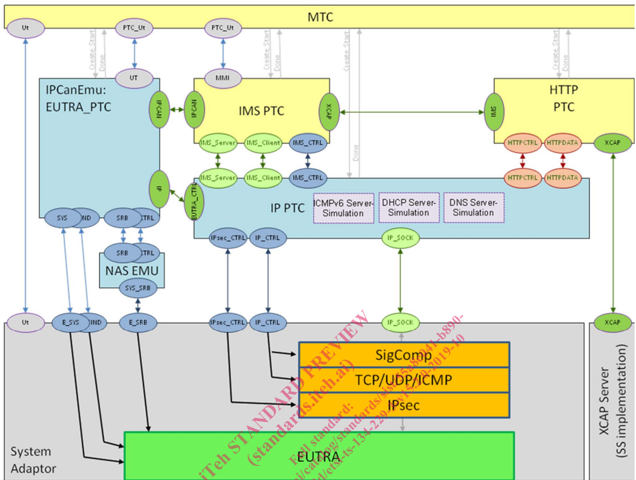
Figure 5.2-1a: Multi-Testers Test Model to support E-UTRA SS interface
