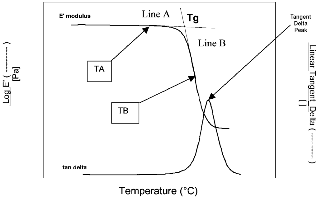
FIG. 1 Construction of Storage Modulus Glass Transition Temperature
