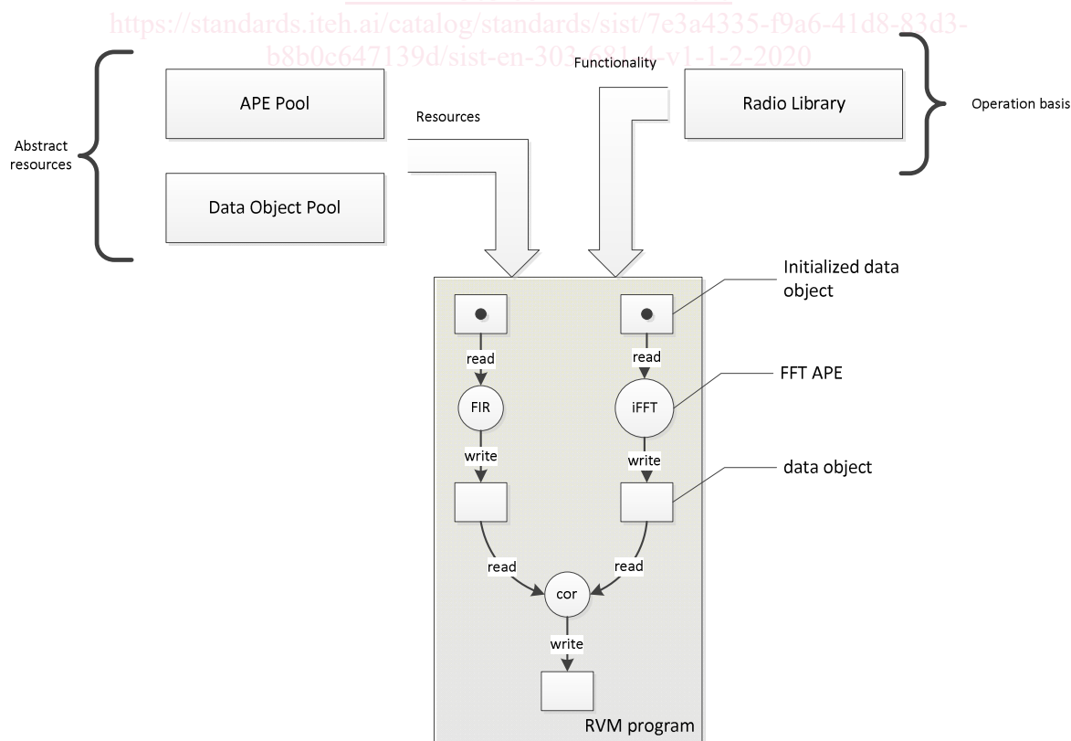
Figure 6.1: Conceptual Diagram of Radio Virtual Machine Processing
