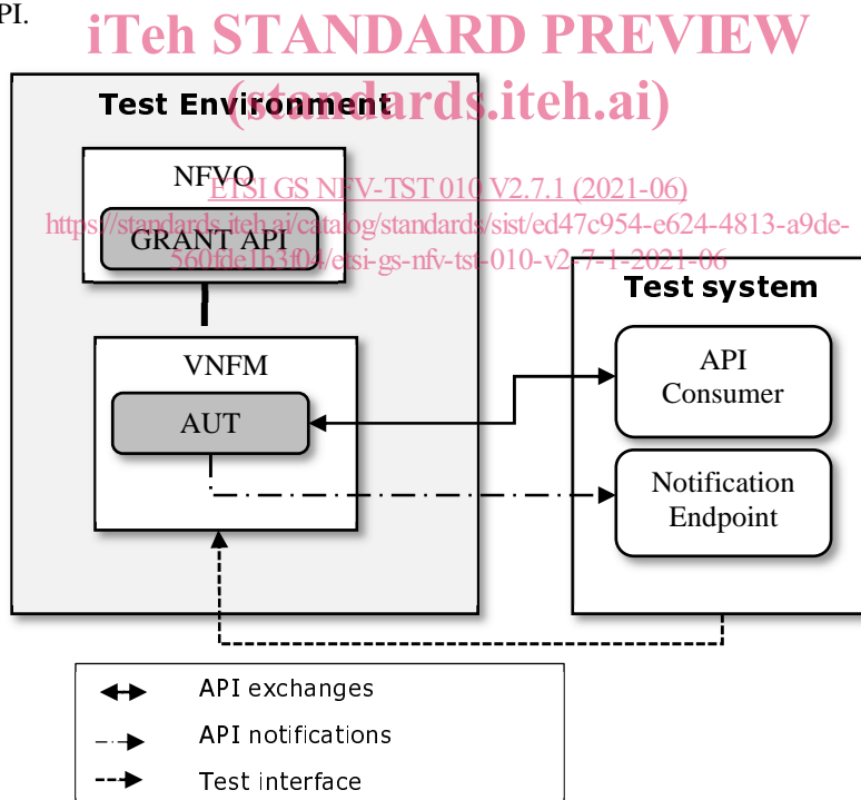
Figure 4.3.5-1: Configuration for tests of APIs with VNFM as Producer, where the VNFLifecycleOperationGranting API is required
