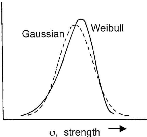
FIG. 2 The Probability Density Function Graphs for Weibull and Gaussian (Normal) Strength Distributions
