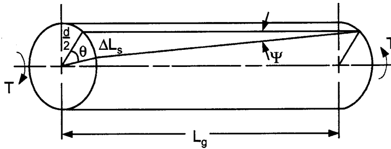
FIG. 1 Twisted Gauge Section of a Cylindrical Specimen Due to a Torsional Moment
