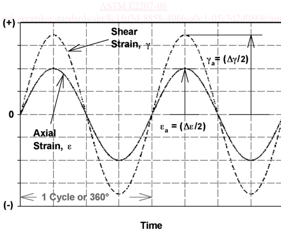
FIG. 2 Schematics of Axial and Shear Strain Waveforms for In- and Out-of-Phase Axial-Torsional Tests
