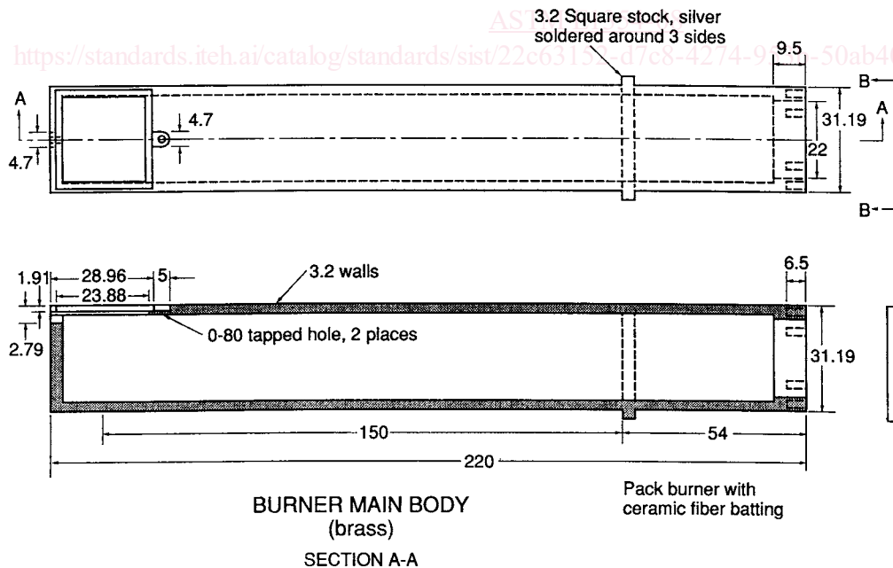
FIG. 11 Calibration Burner
