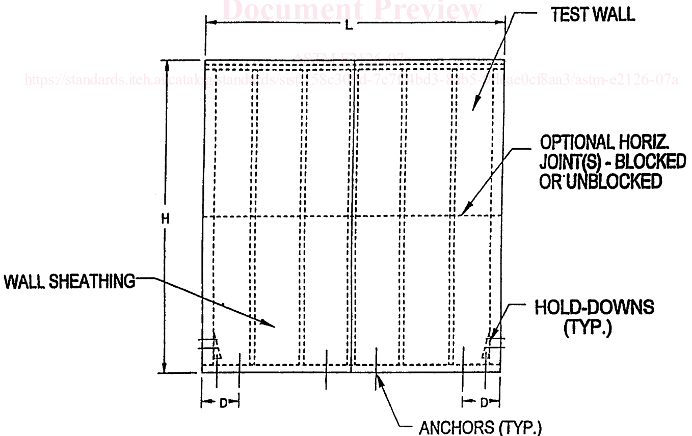
FIG. 3 Example of a Shear Wall Test Specimen
