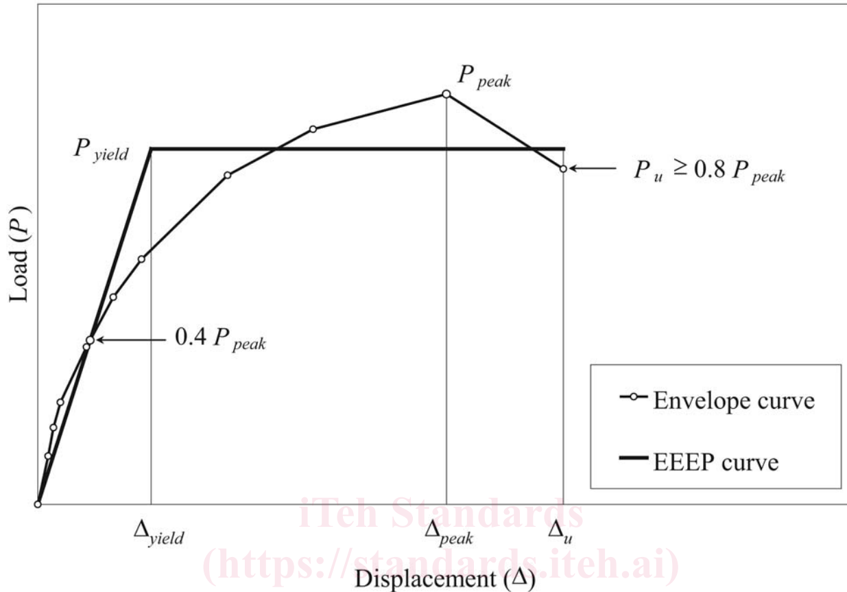
FIG. 2 Performance Parameters of Shear-Wall Assemblies: (A) Last Point at P_u \geq 0.8 P_{peak}
