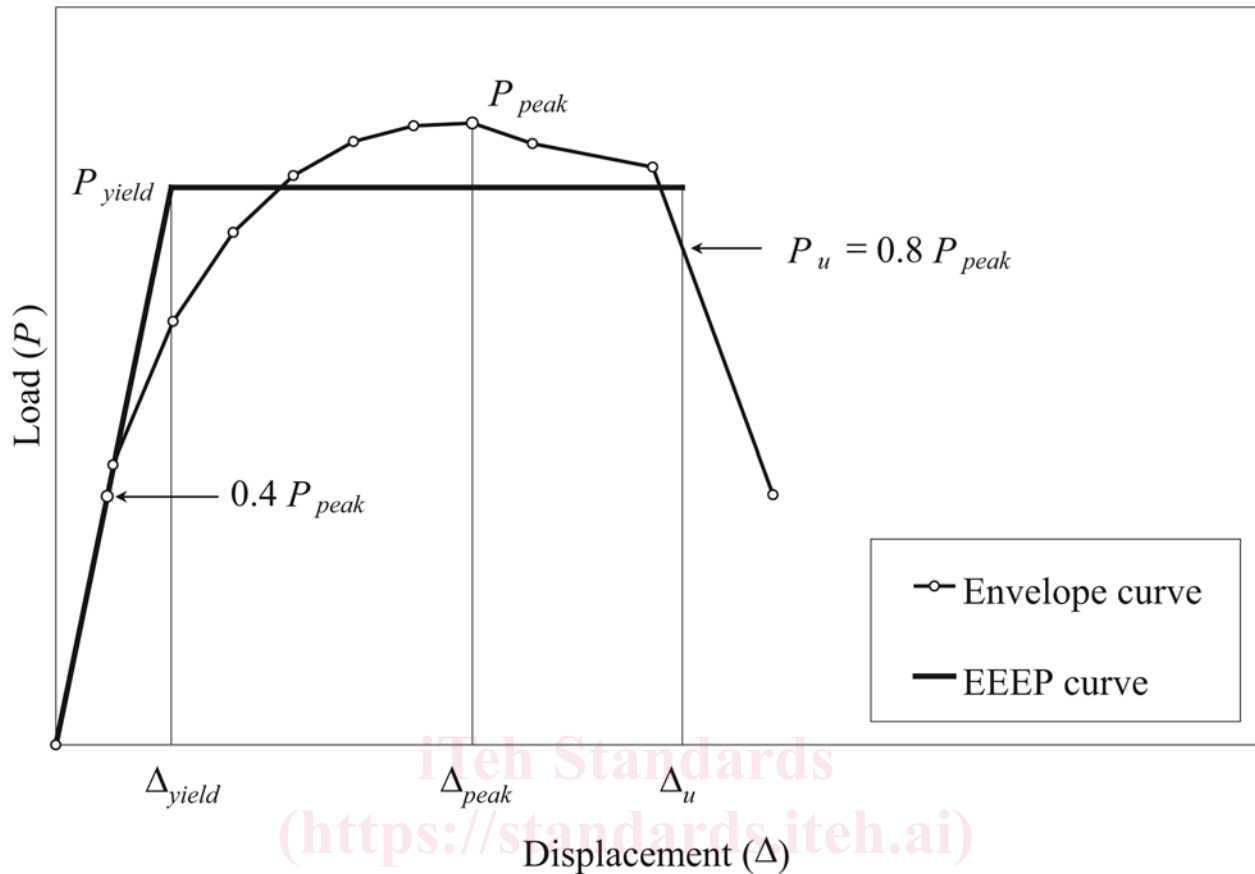
FIG. 2 Performance Parameters of Shear-Wall Assemblies: (B) Last Point at P_u = 0.8 P_{peak} (continued)
