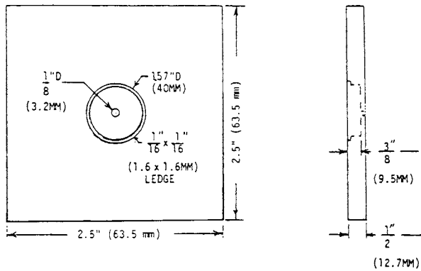
SENSOR SUPPORT OF SOFT INSULATION BOARD
