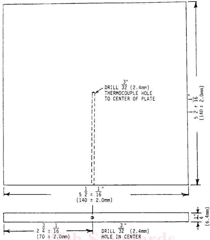
FIG. 2 Surface Plate
