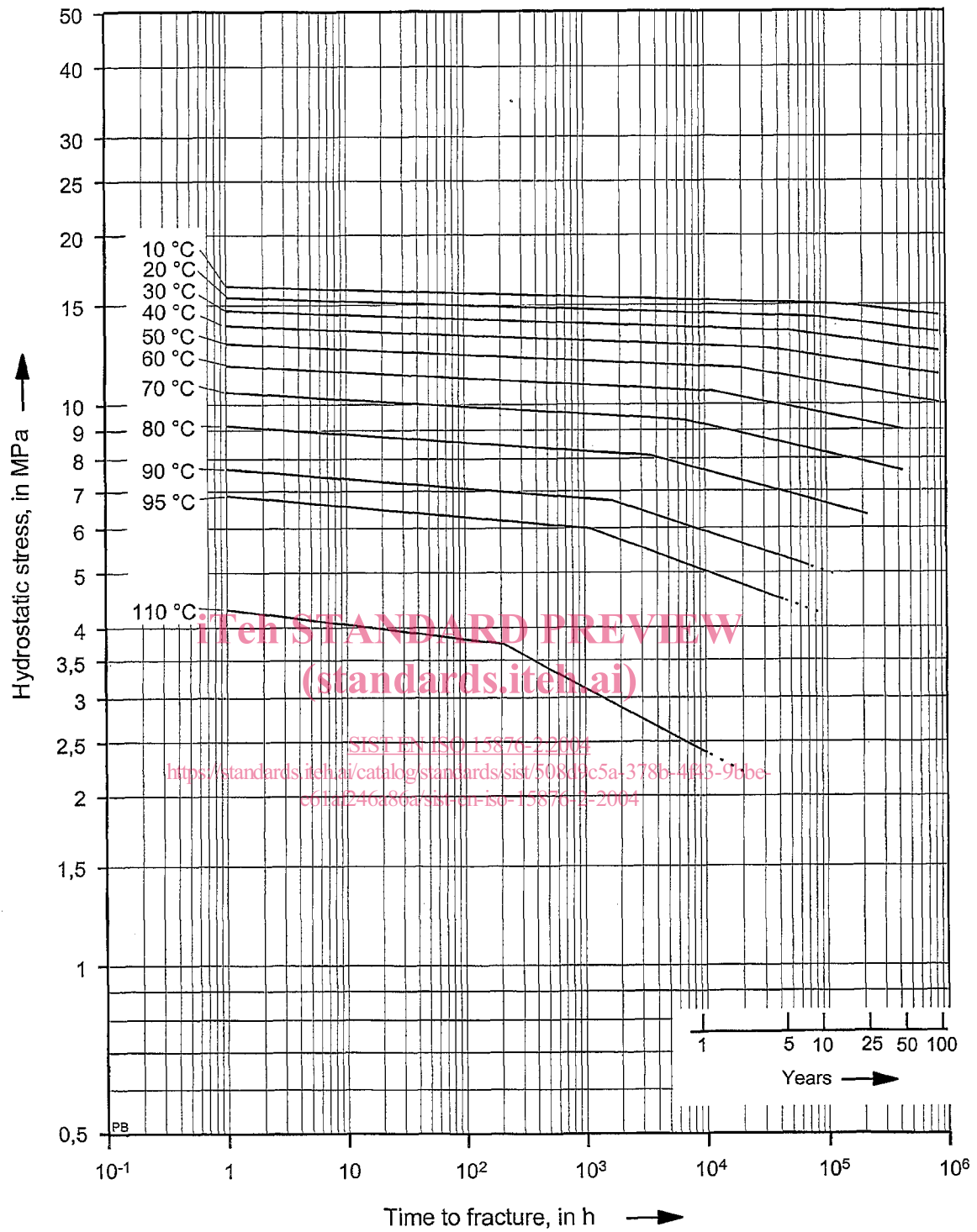
Figure 1 — Reference curves for expected strength of polybutylene
