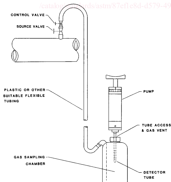
FIG. 1 Apparatus Schematic
